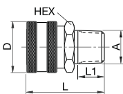
Male Thread
